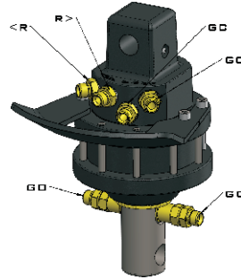
SQUARE HEAD WITH PLATE HOSE GUARD
